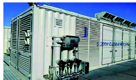
Energy Storage Peaking Station Central de regulação de ponta
